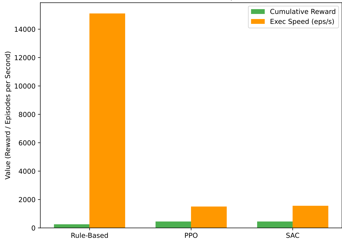
Performance Metrics (500 Episodes)
